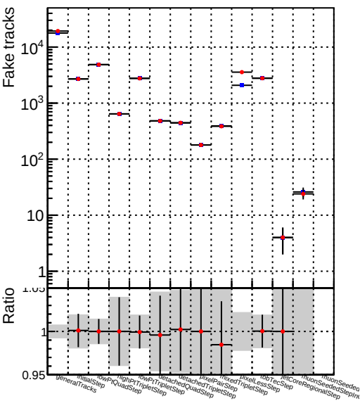
Number —●— DQM_TT_newbranch_time_pLess
