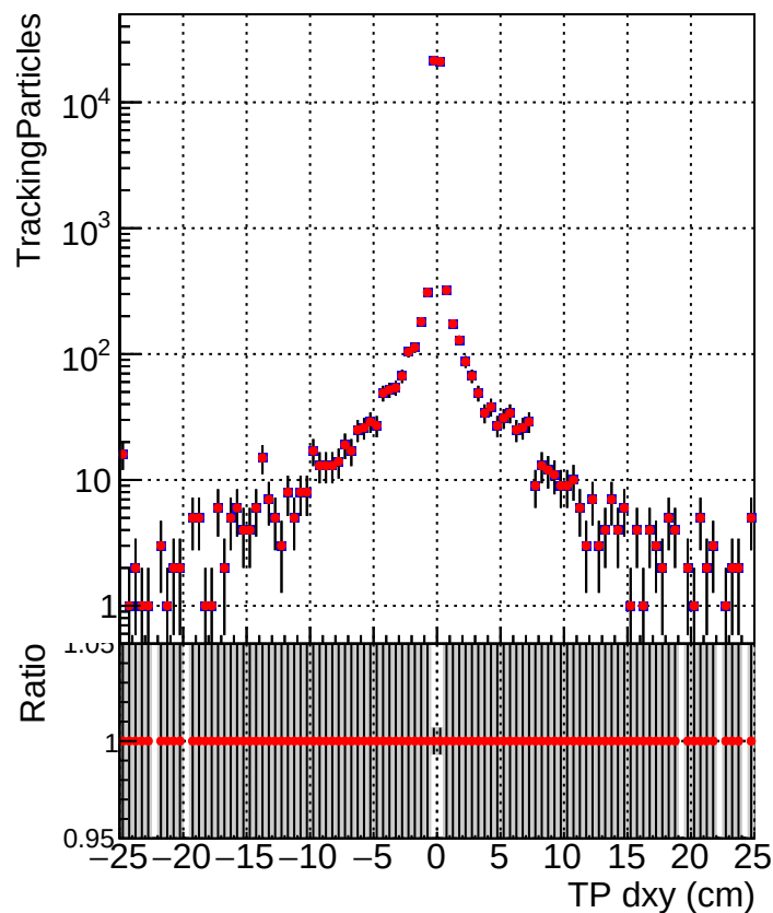
■ DQM_TT_time_newbranch ■ DQM_TT_newbranch_time_pLess
