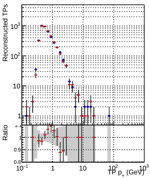
—•— DQM_TT_time_newbranch —•— DQM_TT_newbranch_time_pLess
