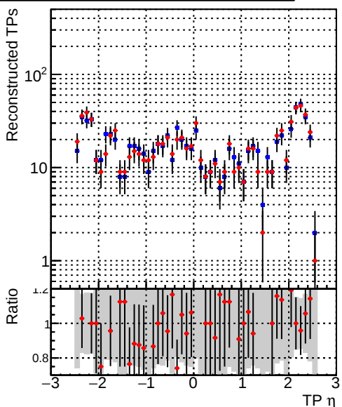
—•— DQM_TT_time_newbranch —•— DQM_TT_newbranch_time_pLess
