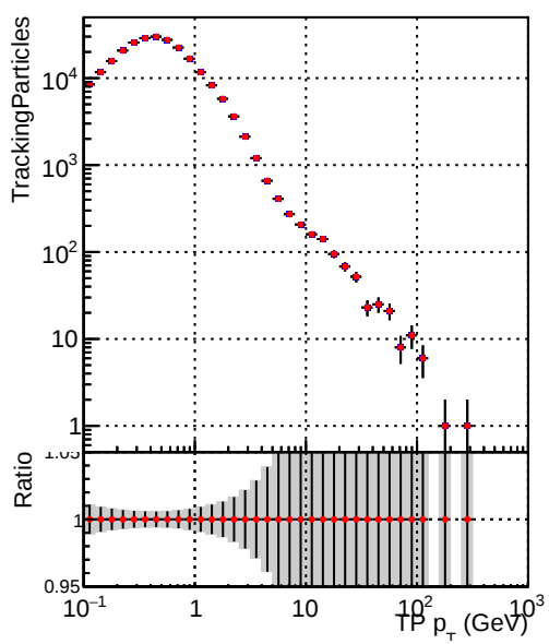
—•— DQM_TT_time_newbranch —•— DQM_TT_newbranch_time_pLess
