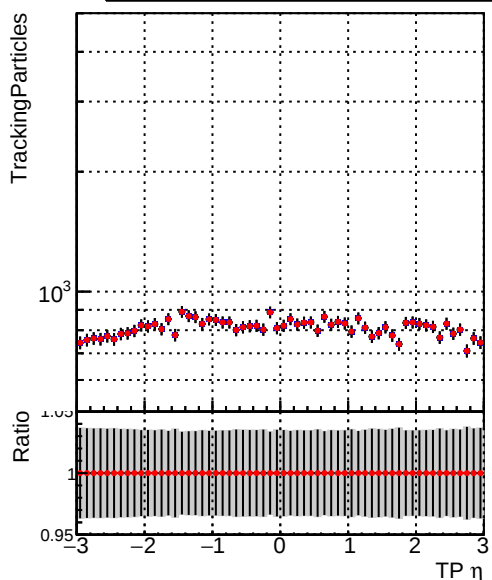
—•— DQM_TT_time_newbranch —•— DQM_TT_newbranch_time_pLess
