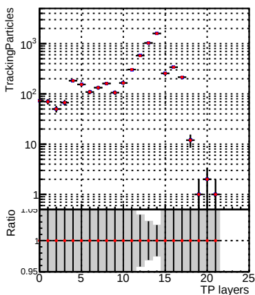
N of sim DQM_TT_newbranch_time_pLess 1000 0.000000 2000 0.000000 3000 0.000000 4000 0.000000 5000 0.000000 6000 0.000000 7000 0.000000 8000 0.000000 9000 0.000000 10000 0.000000 11000 0.000000 12000 0.000000 13000 0.000000 14000 0.000000 15000 0.000000 16000 0.000000 17000 0.000000 18000 0.000000 19000 0.000000 20000 0.000000 21000 0.000000 22000 0.000000 23000 0.000000 24000 0.000000 25000 0.000000 26000 0.000000 27000 0.000000 28000 0.000000 29000 0.000000 30000 0.000000 31000 0.000000 32000 0.000000 33000 0.000000 34000 0.000000 35000 0.000000 36000 0.000000 37000 0.000000 38000 0.000000 39000 0.000000 40000 0.000000 41000 0.000000 42000 0.000000 43000 0.000000 44000 0.000000 45000 0.000000 46000 0.000000 47000 0.000000 48000 0.000000 49000 0.000000 50000 0.000000 51000 0.000000 52000 0.000000 53000 0.000000 54000 0.000000 55000 0.000000 56000 0.000000 57000 0.000000 58000 0.000000 59000 0.000000 60000 0.000000 61000 0.000000 62000 0.000000 63000 0.000000 64000 0.000000 65000 0.000000 66000 0.000000 67000 0.000000 68000 0.000000 69000 0.000000 70000 0.000000 71000 0.000000 72000 0.000000 73000 0.000000 74000 0.000000 75000 0.000000 76000 0.000000 77000 0.000000 78000 0.000000 79000 0.000000 80000 0.000000 81000 0.000000 82000 0.000000 83000 0.000000 84000 0.000000 85000 0.000000 86000 0.000000 87000 0.000000 88000 0.000000 89000 0.000000 90000 0.000000 91000 0.000000 92000 0.000000 93000 0.000000 94000 0.000000 95000 0.000000 96000 0.000000 97000 0.000000 98000 0.000000 99000 0.000000 100000 0.000000
