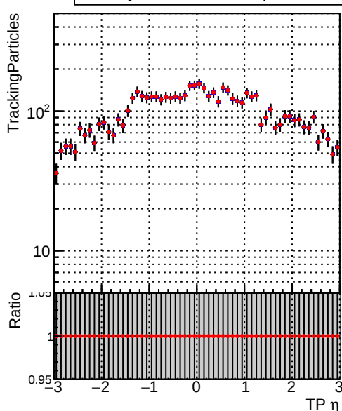
N of simulated tracks vs TP \eta Legend: DQM_TT_time_newbranch (blue dots), DQM_TT_newbranch_time_pLess (red dots)
