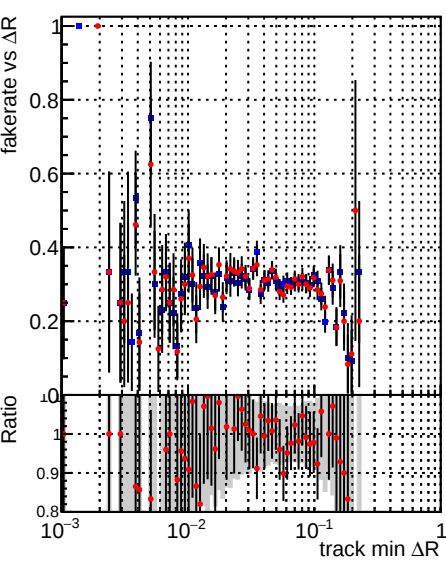
Fake rate vs \Delta R(\text{track, jet}) Legend: \Delta R(\text{track, jet}) (blue), \Delta R(\text{track, jet}) (red)
