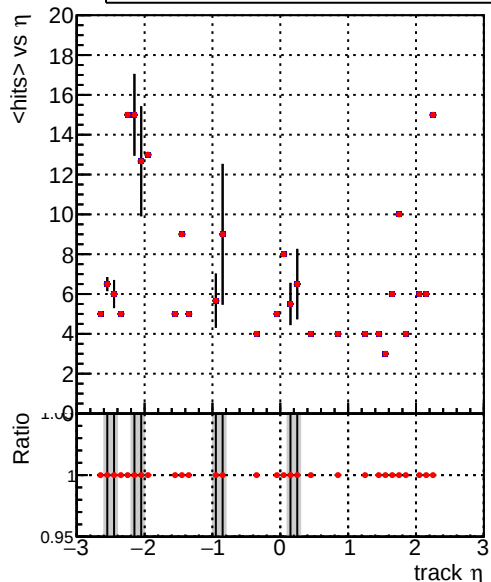
— DQM_TT_time_newbranch — DQM_TT_newbranch_time_pLess
