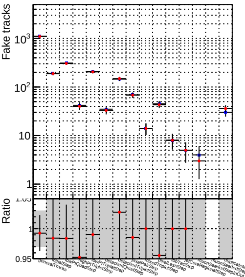
Number —●— DQM_TT_newbranch_time_pLess
