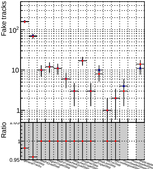
Number —●— DQM_TT_newbranch_time_pLess
