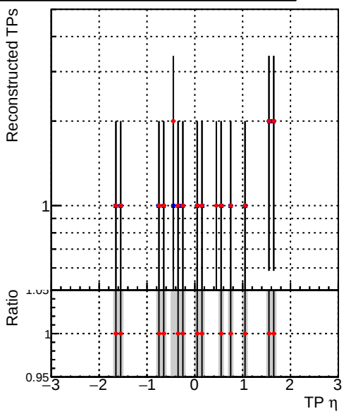
Legend: — DQM_TT_time_newbranch (blue line) — DQM_TT_newbranch_time_pLess (red line)
