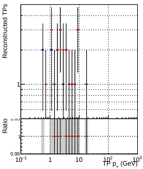
Legend: — DQM_TT_time_newbranch (blue line) — DQM_TT_newbranch_time_pLess (red line)
