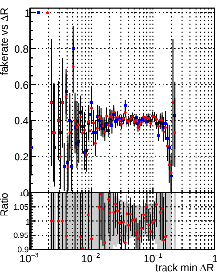
Fake rate vs \Delta R(\text{track, jet}) DQM_TT_time_newbranch DQM_TT_newbranch_time_pLess
