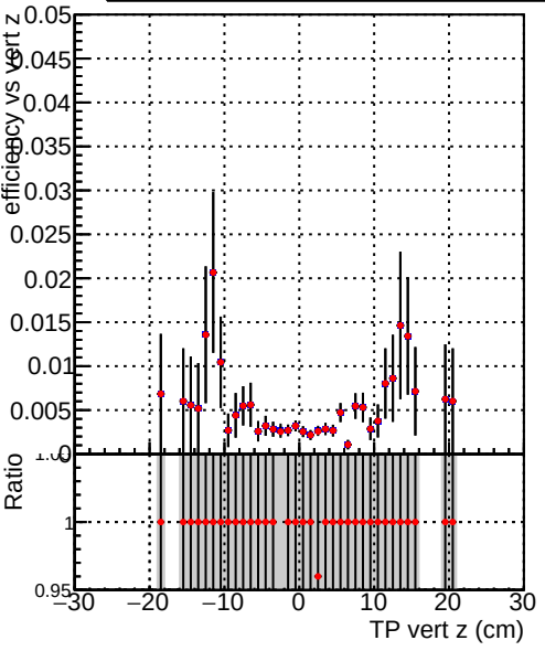
Efficiency vs TP vert z (cm) Legend: DQM_TT_Original (blue line), DQM_TT_Original-pLess (red line)
