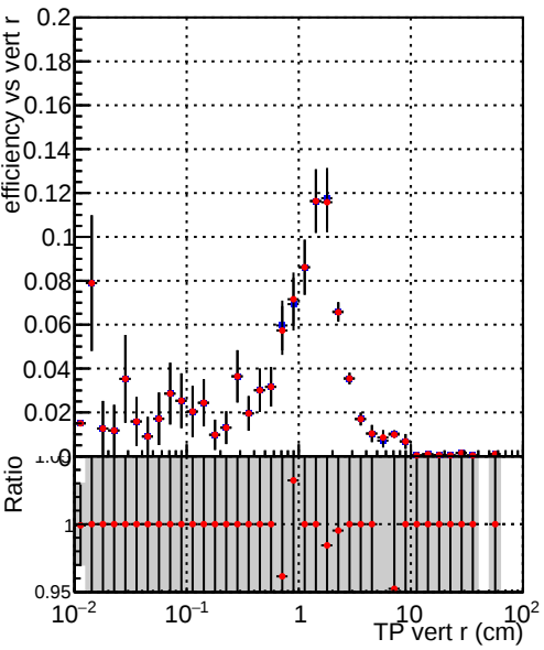
Efficiency vs vertpos Legend: DQM_TT_Original (blue line), DQM_TT_Original-pLess (red line)
