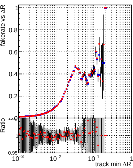
Fake rate vs \Delta R (track, jet) DQM_TT_Original DQM_TT_Original-pLess
