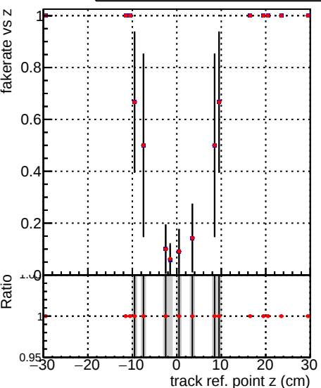
Fake rate vs v DQM_TT_Original DQM_TT_Original-pLess
