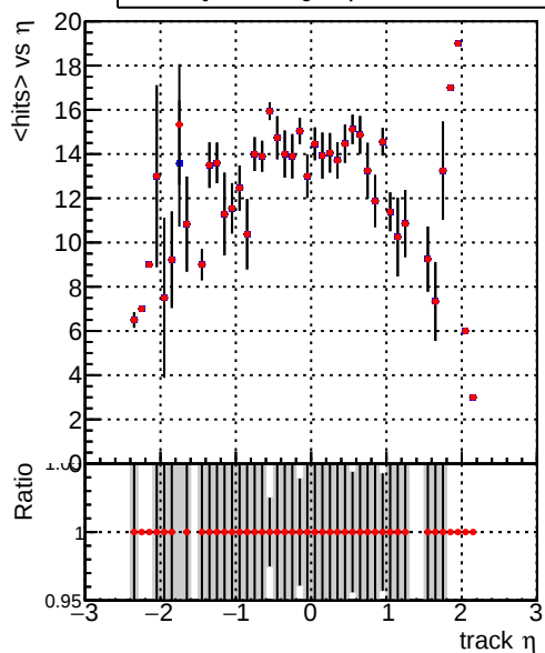
mean hits vs \eta Legend: DQM_TT_Original (blue line), DQM_TT_Original-pLess (red line)
