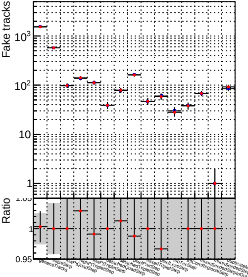
Number —●— DQM_TT_Original-pLess
