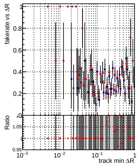
Fake rate vs \Delta R(\text{track, jet}) DQM_TT_Original (blue squares) DQM_TT_Original-pLess (red circles)
