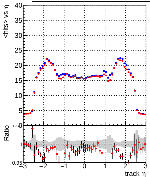
mean hits — DQM_TT_Original — DQM_TT_Original-pLess
