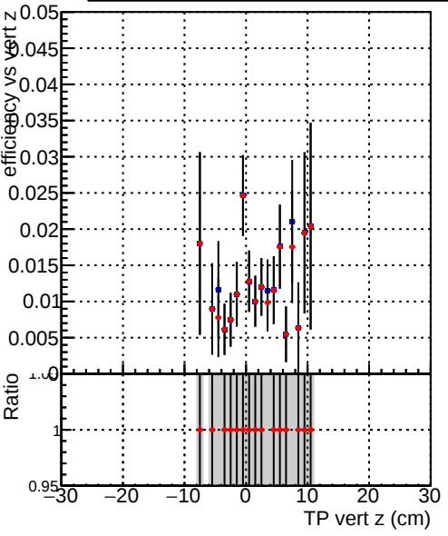
Efficiency vs TP vert z (cm) Legend: DQM_TT_Original DQM_TT_Original-pLess
