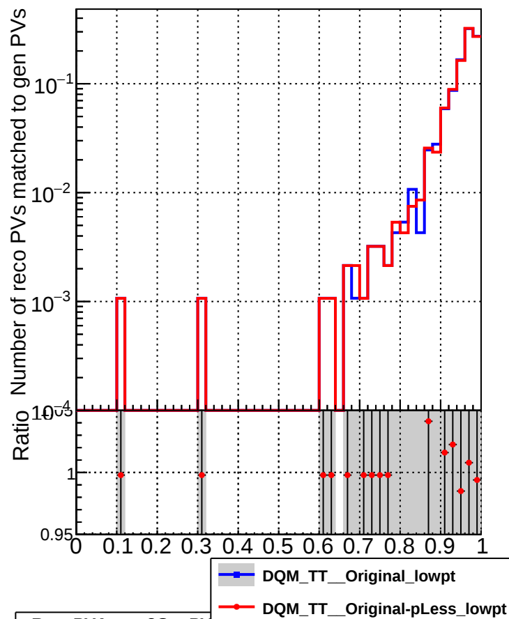
RecoPVAssoc2GenPVMatched_missing
