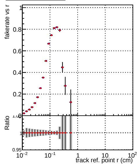
—•— DQM_TT_Original_lowpt —•— DQM_TT_Original-pLess_lowpt
