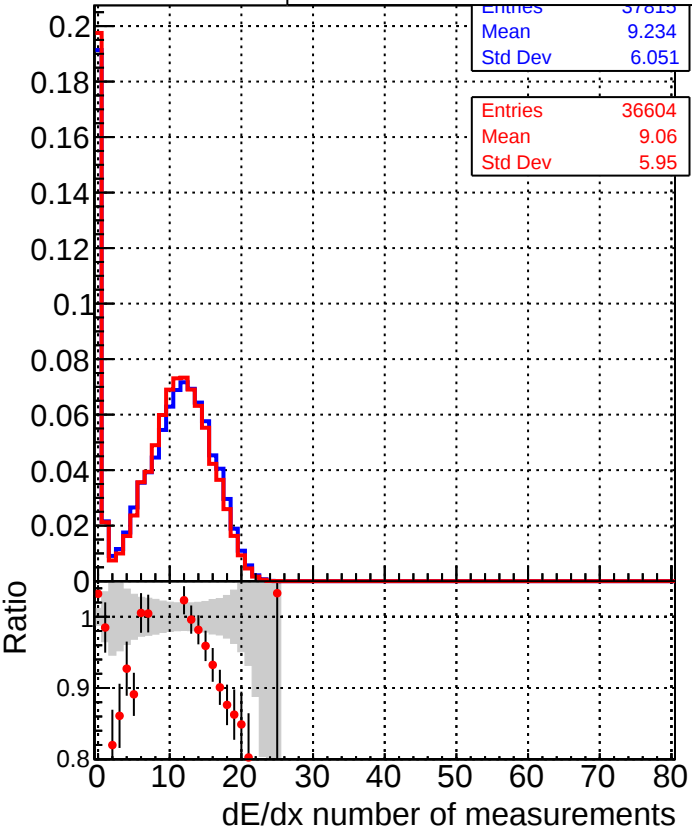
■ DQM_TT_Original_lowpt ● DQM_TT_Original-pLess_lowpt
