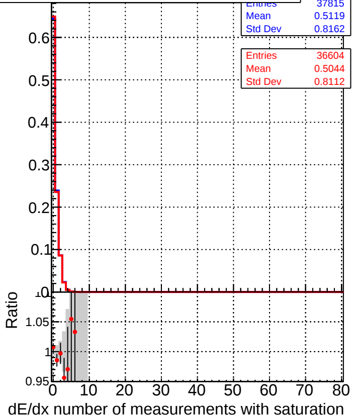
■ DQM_TT_Original_lowpt ● DQM_TT_Original-pLess_lowpt
