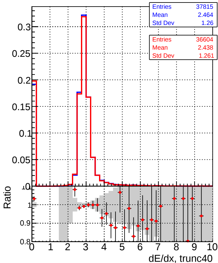
■ DQM_TT_Original_lowpt ● DQM_TT_Original-pLess_lowpt
