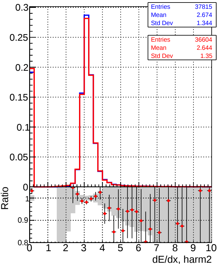
■ DQM_TT_Original_lowpt ● DQM_TT_Original-pLess_lowpt
