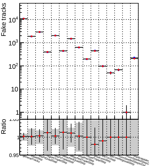
Number —●— DQM_TT_Original-pLess_lowpt
