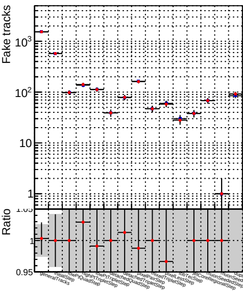
Number —●— DQM_TT_Original-pLess_lowpt
