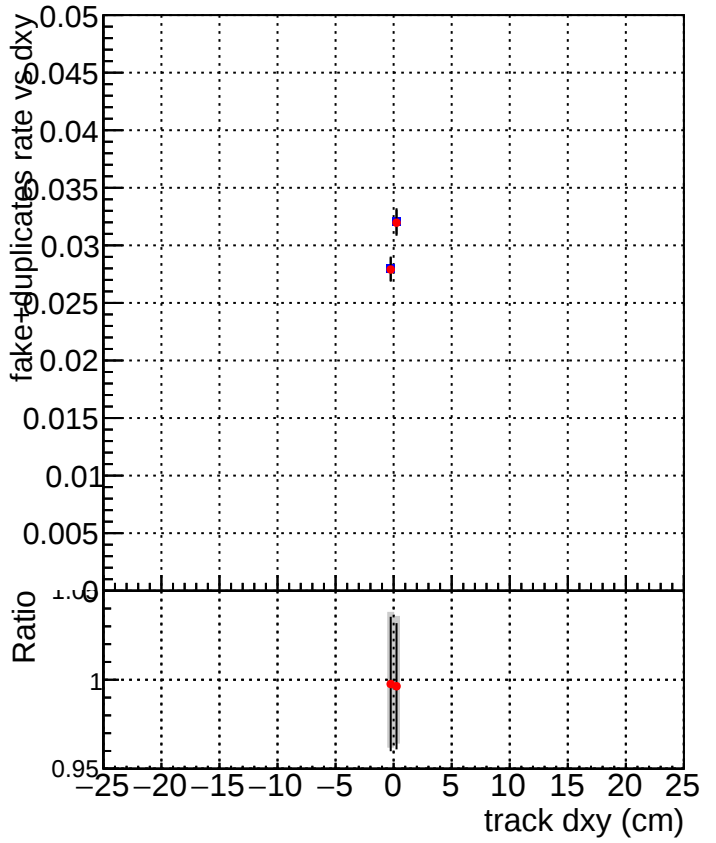
DQM_TT_Original_lowpt DQM_TT_Original-pLess_lowpt
