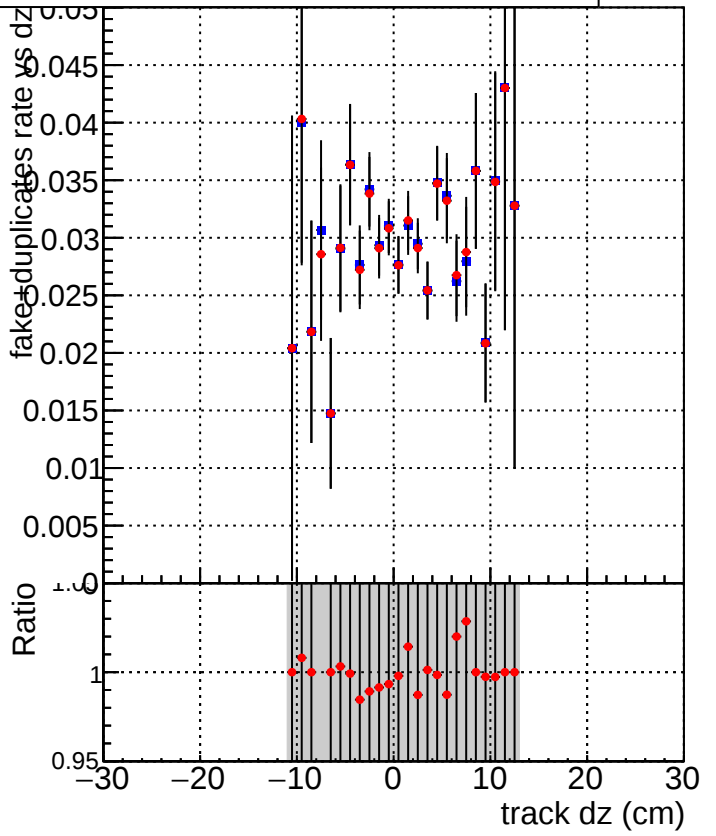
DQM_TT_Original_lowpt DQM_TT_Original-pLess_lowpt
