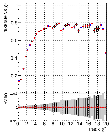
Fake rate vs. —●— DQM TT Original_lowpt —●— DQM TT Original-pLess_lowpt
