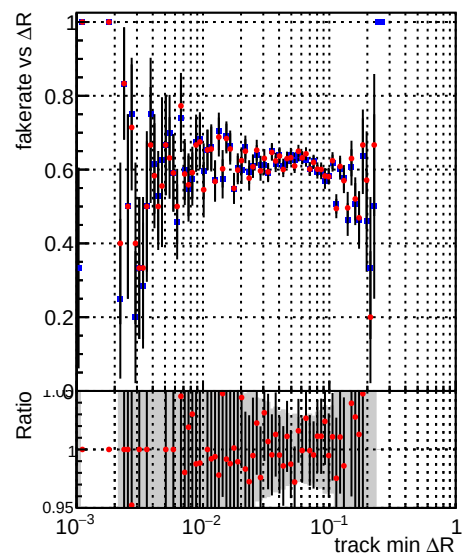
—■— DQM_TT_Original_lowpt —●— DQM_TT_Original-pLess_lowpt
