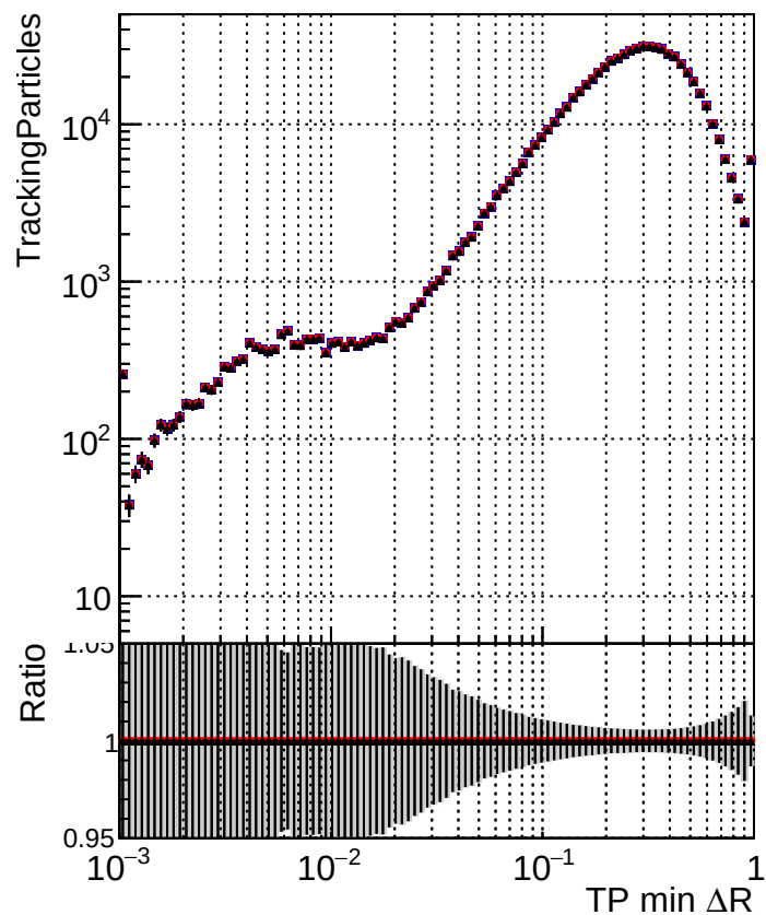
N of simulated tracks vs dR ■ DQM_XiMinus_original_lowpt ● DQM_XiMinus_newbranch_lowpt_pLess ▲ DQM_XiMinus_newbranch_lowpt_pLessMVACand
