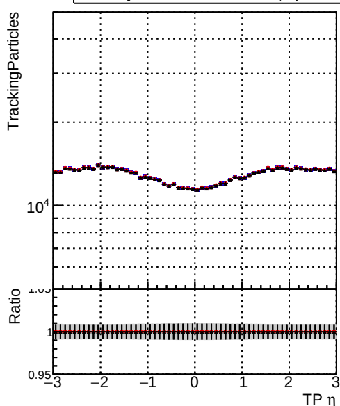
—•— DQM_XiMinus_original_lowpt —•— DQM_XiMinus_newbranch_lowpt_pLess —•— DQM_XiMinus_newbranch_lowpt_pLessMVAand
