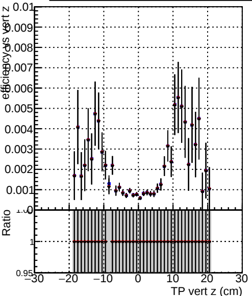
Efficiency vs vertpos DQM_XiMinus_original_lowpt DQM_XiMinus_newbranch_lowpt_pLess DQM_XiMinus_newbranch_lowpt_pLessMVACand
