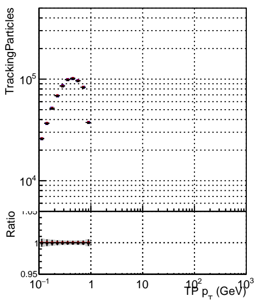
Legend: DQM_XiMinus_original_lowpt (blue circles), DQM_XiMinus_newbranch_lowpt_pLess (red circles), DQM_XiMinus_newbranch_lowpt_pLessMVACand (black circles)
