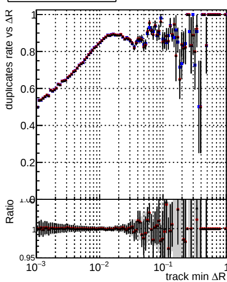
—•— DQM_XiMinus_original_lowpt —•— DQM_XiMinus_newbranch_lowpt_pLess —•— DQM_XiMinus_newbranch_lowpt_pLessMVACand
