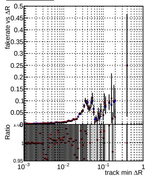
—•— DQM_XiMinus_original_lowpt —•— DQM_XiMinus_newbranch_lowpt_pLess —•— DQM_XiMinus_newbranch_lowpt_pLessMVACand
