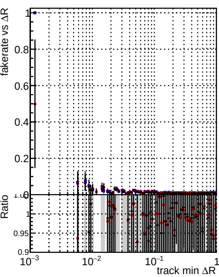
Legend: DQM XiMinus original_lowpt (blue squares), DQM XiMinus newbranch_lowpt_pLess (red circles), DQM XiMinus newbranch_lowpt_pLessMVACand (black crosses)
