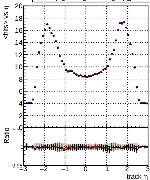
mean hits vs \eta — DQM_XiMinus_original_lowpt — DQM_XiMinus_newbranch_lowpt_pLess — DQM_XiMinus_newbranch_lowpt_pLessMVACand
