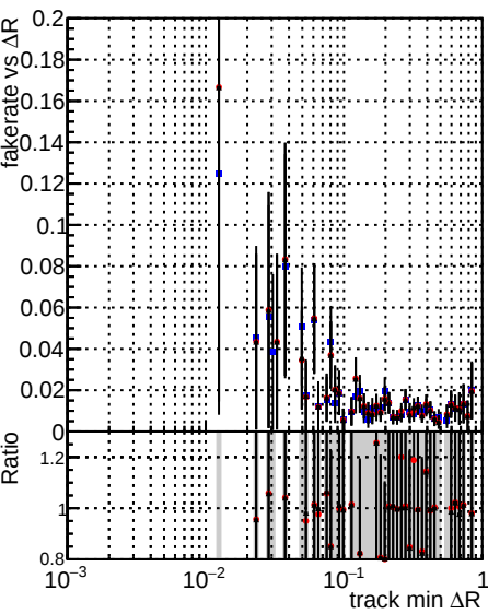
Fake rate vs ΔR(track, jet) Legend: DQM_XiMinus_original_lowpt (black line with blue dots) DQM_XiMinus_newbranch_lowpt_pLess (red line with red dots) DQM_XiMinus_newbranch_lowpt_pLessMVACand (black line with black dots)
