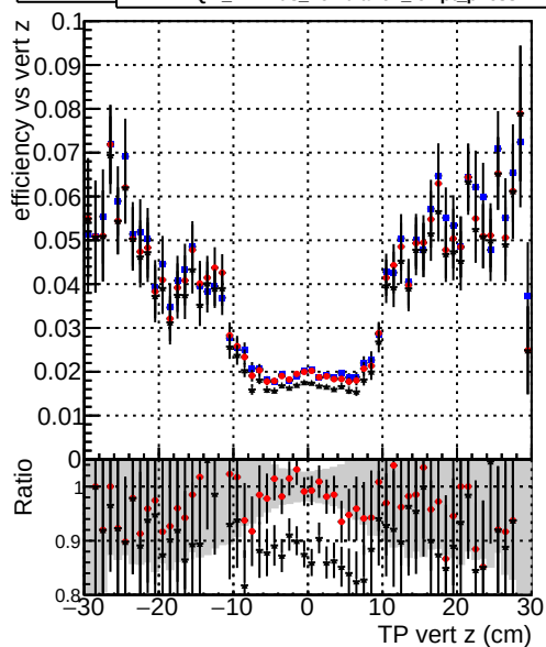
Efficiency —●— DQM_XiMinus_original_lowpvt —●— DQM_XiMinus_newbranch_lowpvt_pLess —●— DQM_XiMinus_newbranch_lowpvt_pLessMVACand
