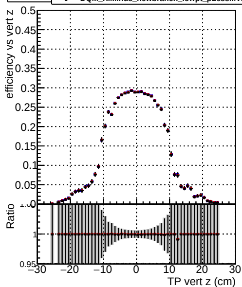
Efficiency vs. sim PV z — DQM_XiMinus_original_lowpt — DQM_XiMinus_newbranch_lowpt_pLess — DQM_XiMinus_newbranch_lowpt_pLessMVAand
