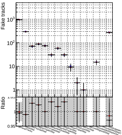
Number Legend 1 DQM_XiMinus_newbranch_lowpt_pLess 2 DQM_XiMinus_newbranch_lowpt_pLessMVACand
