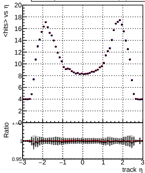
mean hits vs \eta DQM_XiMinus_original_lowpT DQM_XiMinus_newbranch_lowpT_pLess DQM_XiMinus_newbranch_lowpT_pLessMVACand
