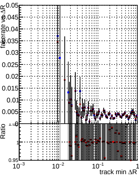
Fake rate vs \Delta R(\text{track, jet}) DQM_XiMinus_original_lowpt DQM_XiMinus_newbranch_lowpt_pLess DQM_XiMinus_newbranch_lowpt_pLessMVACand
