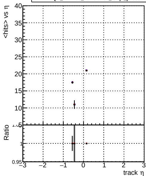
mean hits — DQM_XiMinus_original_lowpt — DQM_XiMinus_newbranch_lowpt_pLess — DQM_XiMinus_newbranch_lowpt_pLessMVACand
