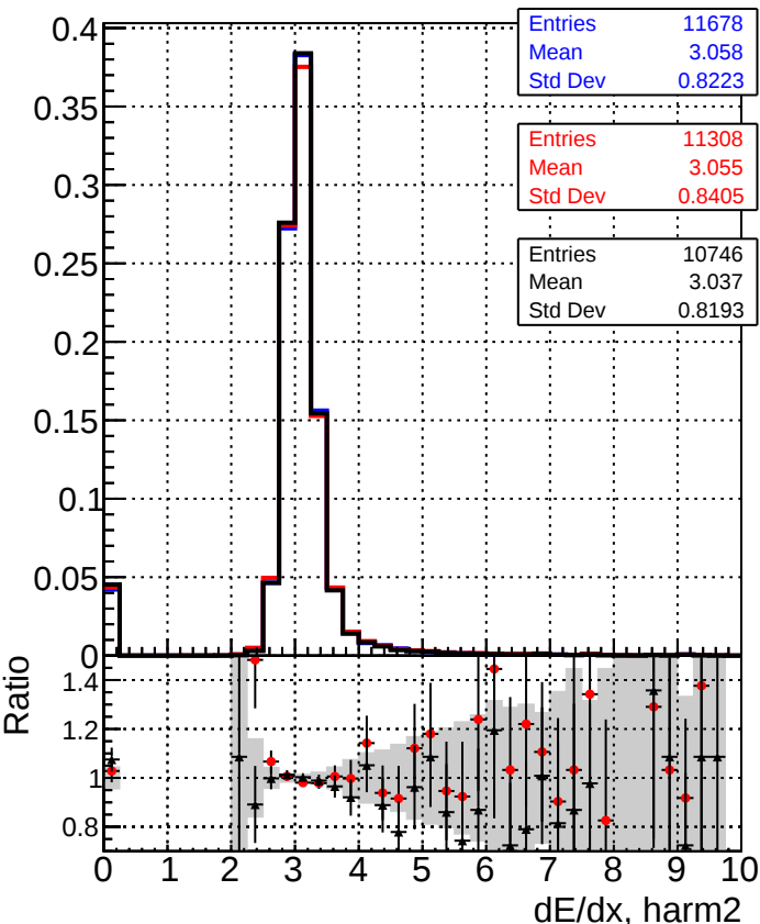
—■— DQM_XiMinus_original_lowpt —●— DQM_XiMinus_newbranch_lowpt_pLess —▲— DQM_XiMinus_newbranch_lowpt_pLessMVACand
