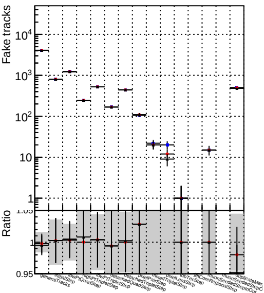
Number ● DQM_XiMinus_newbranch_lowpt_pLess ▲ DQM_XiMinus_newbranch_lowpt_pLessMVA Cand
