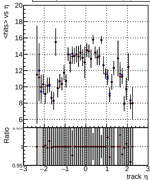
mean hit — DQM_XiMinus_original_lowpt — DQM_XiMinus_newbranch_lowpt_pLess — DQM_XiMinus_newbranch_lowpt_pLessMVACand
