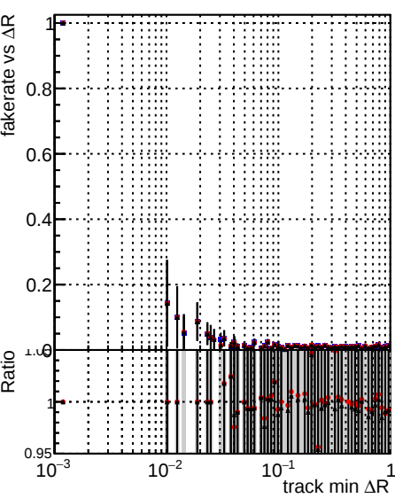
Legend: DQM_XiMinus_original_lowpt (black), DQM_XiMinus_newbranch_lowpt_pLess (red), DQM_XiMinus_newbranch_lowpt_pLessMVACand (grey)
