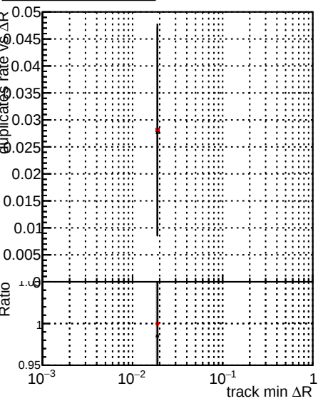
Legend: - \square DQM_XiMinus_original_lowpt - \square DQM_XiMinus_newbranch_lowpt_pLess - \square DQM_XiMinus_newbranch_lowpt_pLessMVACand
