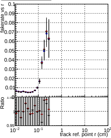
Fake rate vs vertpos —●— DQM_XiMinus_original_lowpt —●— DQM_XiMinus_newbranch_lowpt_pLess —●— DQM_XiMinus_newbranch_lowpt_pLessMVACand
