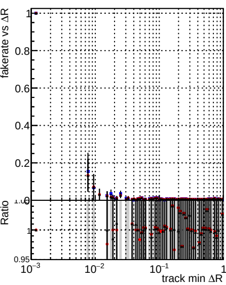
Legend: DOM XiMinus original_lowpt DOM XiMinus newbranch_lowpt_pLess DOM XiMinus newbranch_lowpt_pLessMVACand
