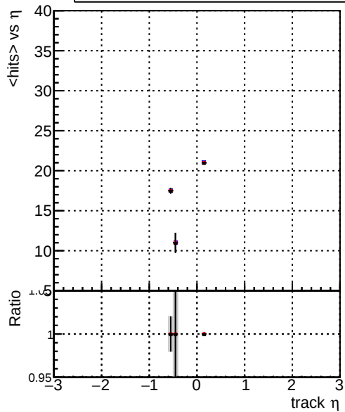
mean hits — DQM_XiMinus_original_lowpt — DQM_XiMinus_newbranch_lowpt_pLess — DQM_XiMinus_newbranch_lowpt_pLessMVAand
